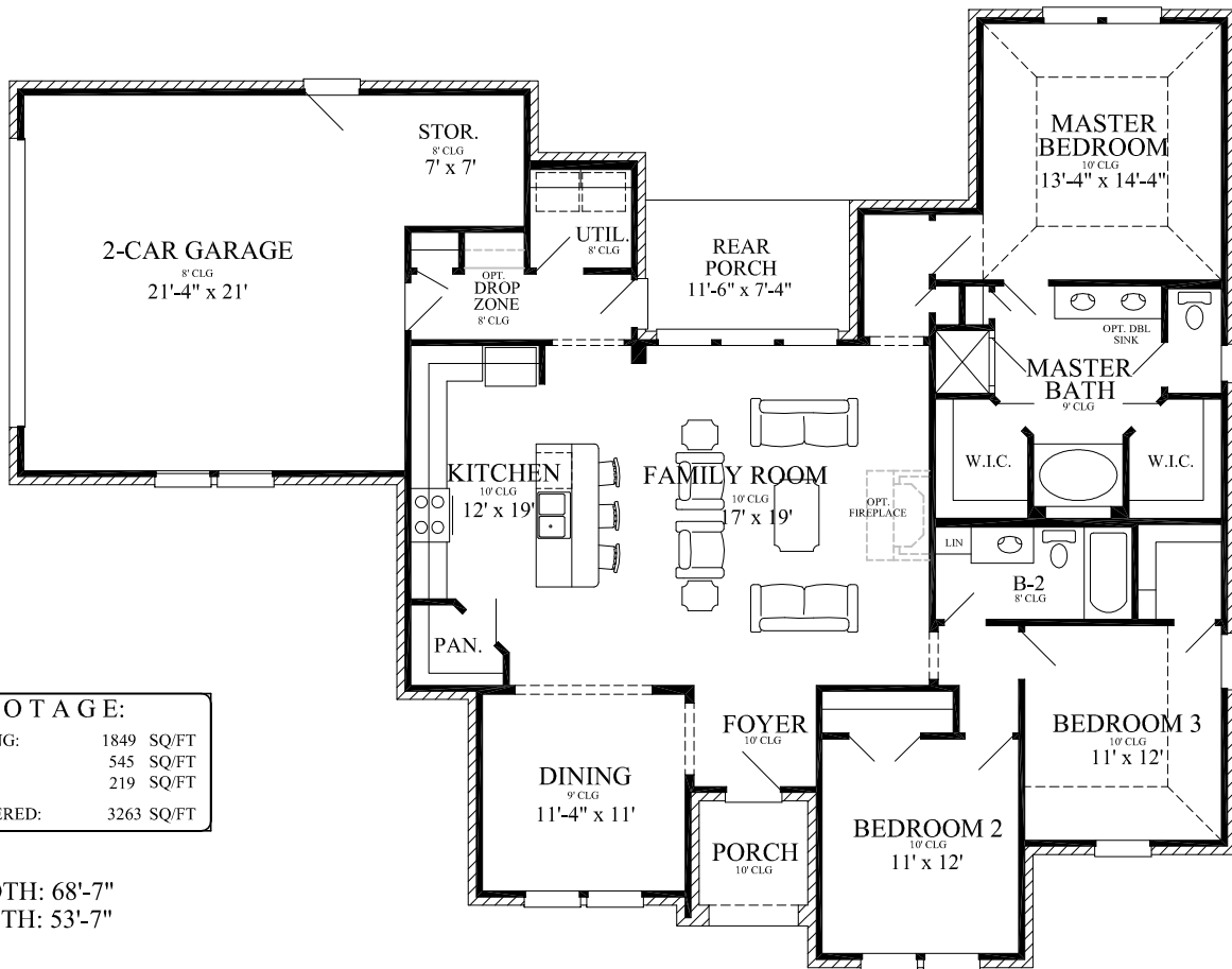
FLOOR PLAN
